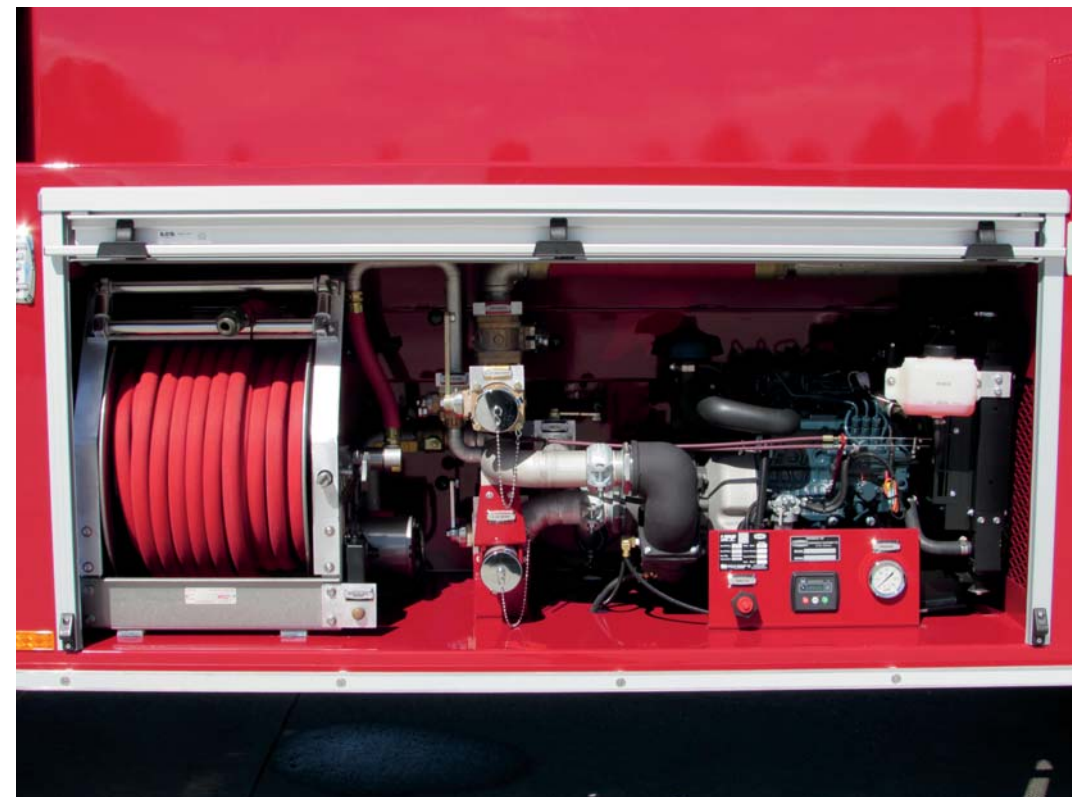
Multiple Pump Configurations: Gas & Diesel Booster Reel Options Available
